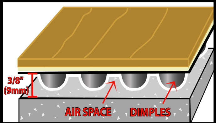
1 Unroll Warm N Quiet Subfloor™ and cut to fit. Leave a 3/8" gap around walls stairs and supports
